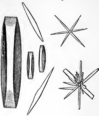
Fig. 14.—CREATININE (after Frey).
